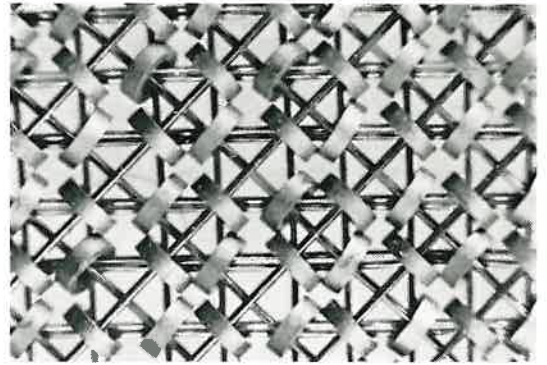
Figure 6 The magnetic core memory. Each element in the magnetic memory consists of a toroid or core of magnetic material having an outside diameter of 0.05in and threaded with four wires. Many thousands of these cores are assembled as a compact matrix. Individual cores can be magnetized in the clockwise or anti-clockwise direction by passing a pulse of current through certain of the linking wires. This magnetic state will persist until reversed by a current pulse in the opposite direction. Data is 'written into' the memory by magnetizing particular cores in a given direction representing the '1' state while the remainder are left in the opposite or '0' state. The memorized data is 'read out' by collectively magnetizing all cores in the '0' state which, of course, involves a reversal of the magnetic flux in such cores as were previously in the '1' state. Each core has its own sensing wire, and a flux reversal causes a current pulse to appear in this wire, enabling the original data to be recovered for use. Since the 'read' process causes all cores to revert to the '0' state, provision is made for the memorized data to be automatically 're-written' after each 'read' cycle.
