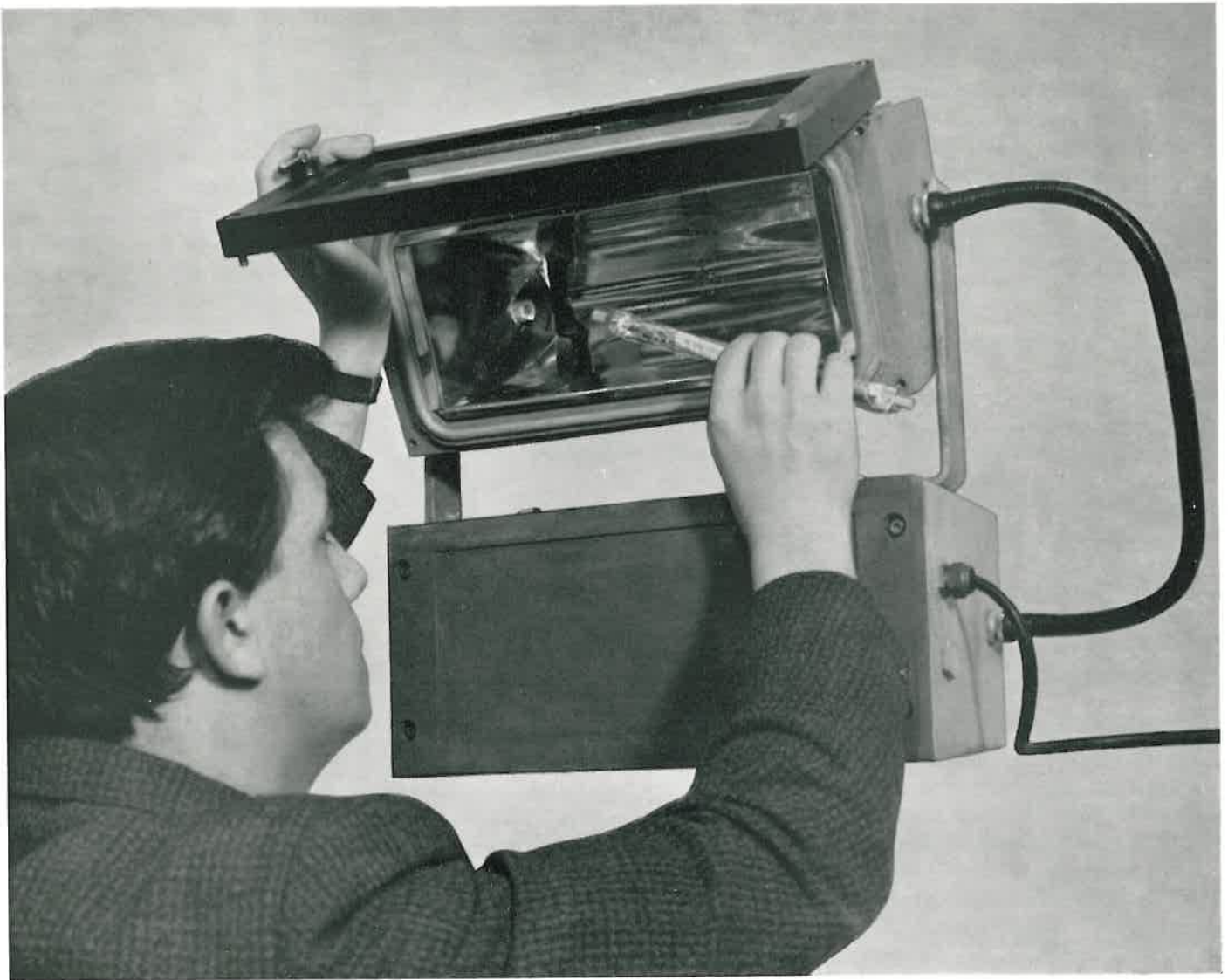
Figure 1 The Mazda linear mercury halide lamp with its associated reflector lantern.
