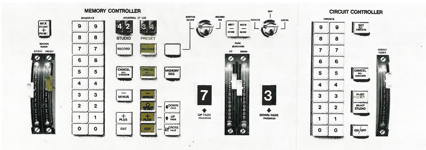
Figure 3 A typical Thorn Q-File control panel layout
