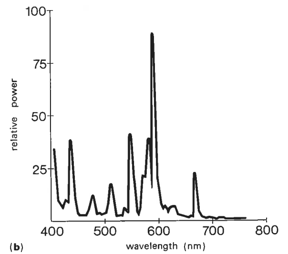
Figure 2 Spectral distribution of power from (a) the high pressure mercury vapour lamp (MB/U) and (b) the linear mercury halide lamp (MBIL/H)
