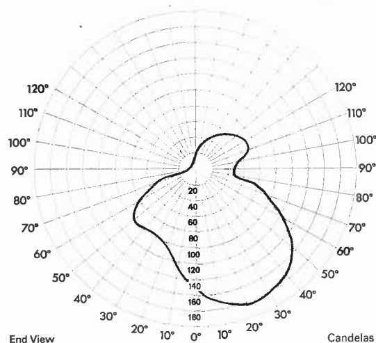
Polar distribution of the Atlas asymmetrical fitting.
