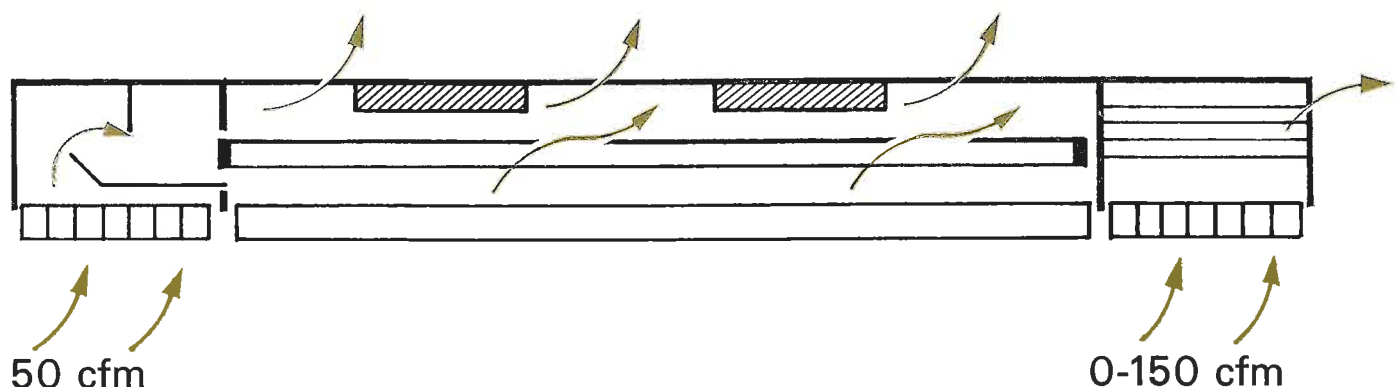
Figure 1 Longitudinal section of fitting showing air flow paths
